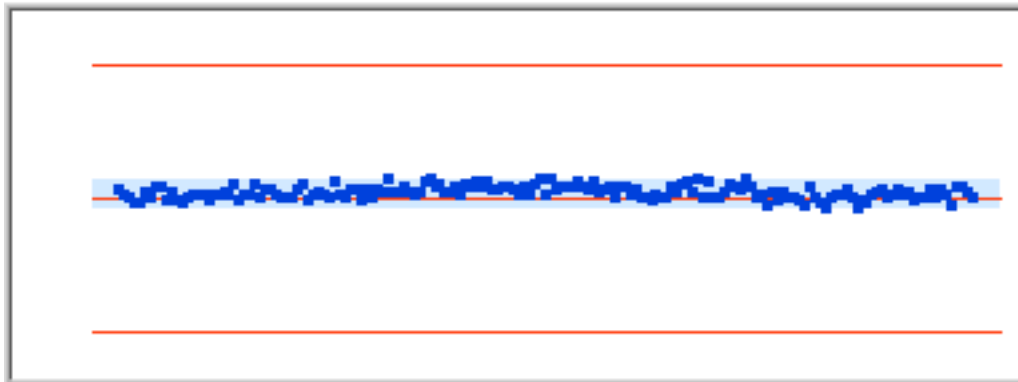
Figure77 Distribution 1833.775Hz
