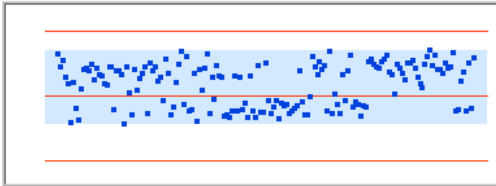
Figure135 Distribution 5005.692Hz
