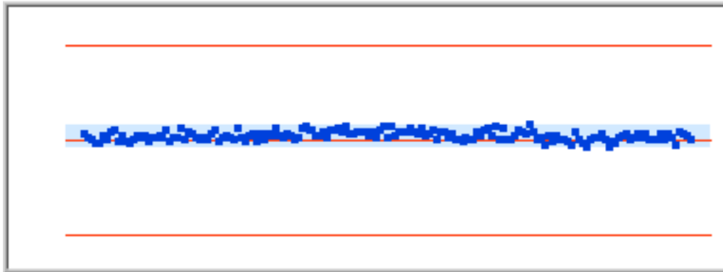
Figure75 Distribution 1771.286Hz
