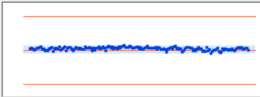
Figure29 Distribution 798.667Hz
