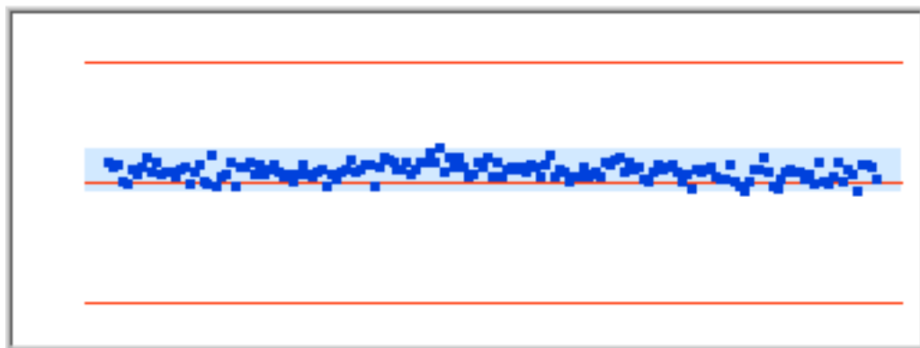
Figure49 Distribution 1129.252Hz
