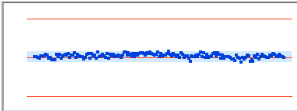
Figure35 Distribution 886.112Hz
