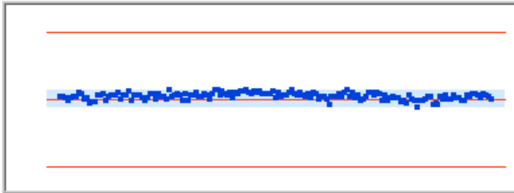
Figure33 Distribution 856.014Hz
