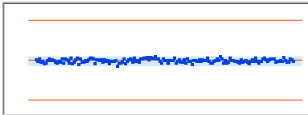
Figure103 Distribution 2876.364Hz
