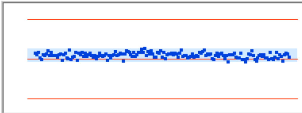
Figure47 Distribution 1090.771Hz
