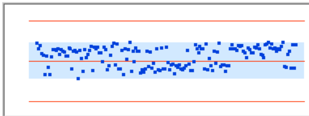
Figure133 Distribution 4835.667Hz
