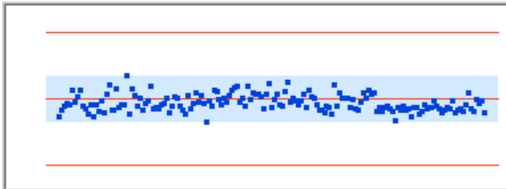
Figure173 Distribution 9665.114Hz
