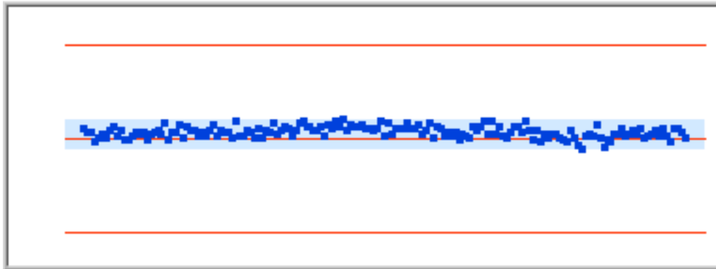
Figure57 Distribution 1296.944Hz
