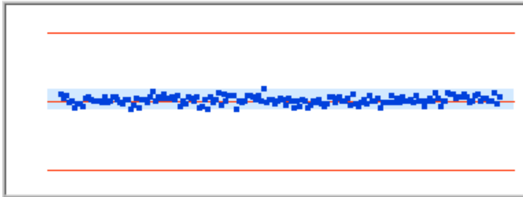
Figure129 Distribution 4511.715Hz
