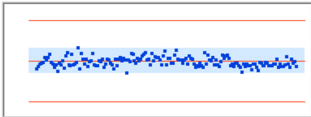
Figure157 Distribution 7326.505Hz
