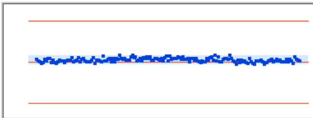
Figure83 Distribution 2034.551Hz
