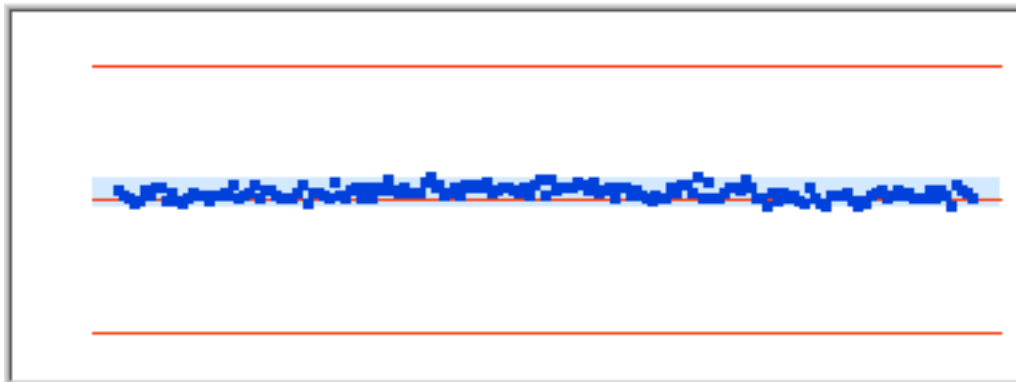
Figure81 Distribution 1965.220Hz
