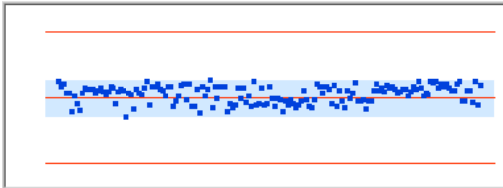
Figure131 Distribution 4670.883Hz
