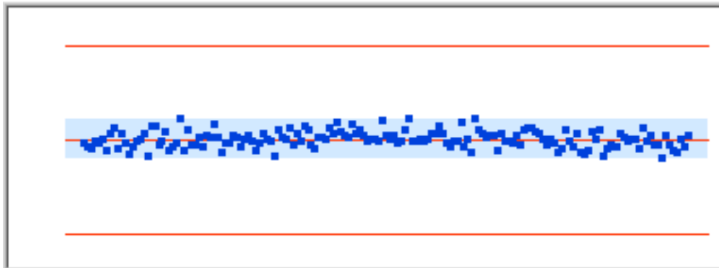
Figure143 Distribution 5749.685Hz
