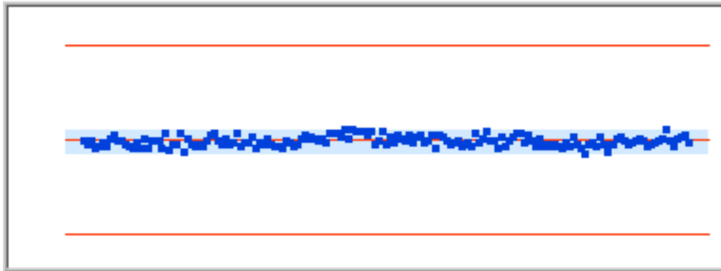
Figure123 Distribution 4066.485Hz
