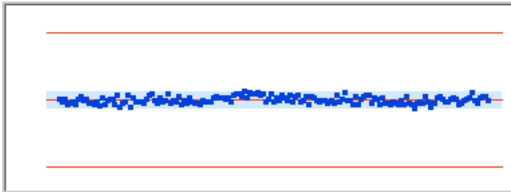
Figure125 Distribution 4209.946Hz
