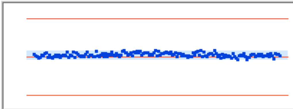
Figure71 Distribution 1652.812Hz
