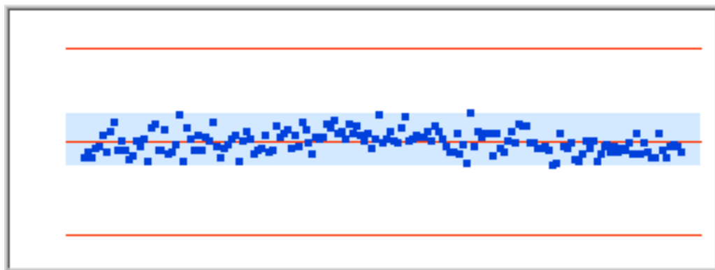
Figure145 Distribution 5951.848Hz
