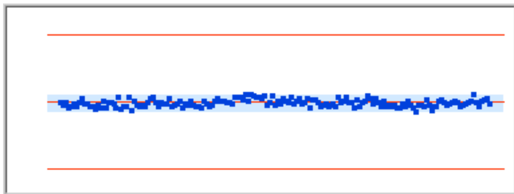
Figure121 Distribution 3928.361Hz
