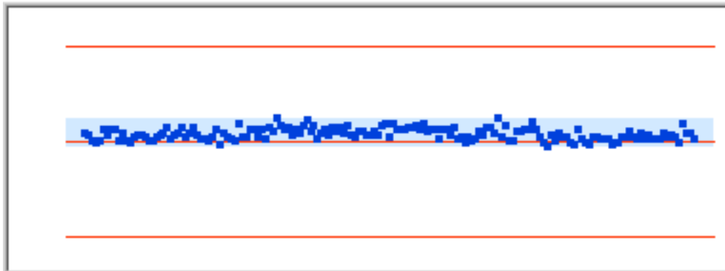
Figure95 Distribution 2504.457Hz
