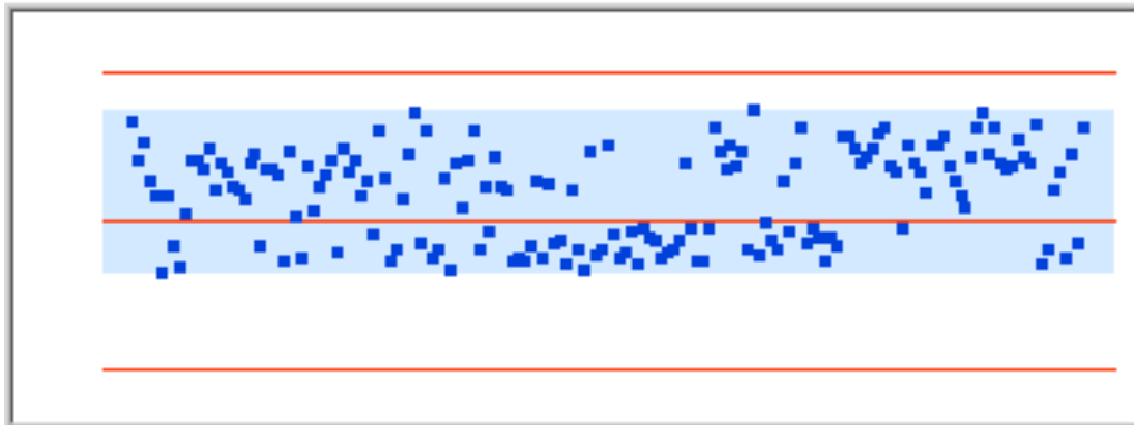
Figure137 Distribution 5182.288Hz
