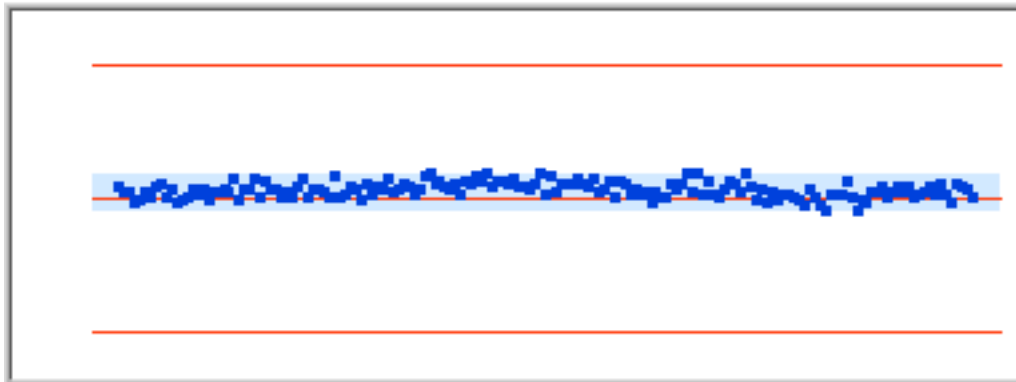
Figure59 Distribution 1342.698Hz
