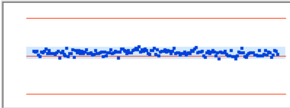
Figure45 Distribution 1053.721Hz
