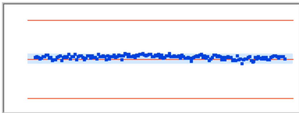
Figure31 Distribution 826.844Hz
