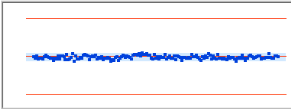
Figure111 Distribution 3303.876Hz
