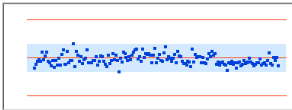
Figure175 Distribution 10006.089Hz
