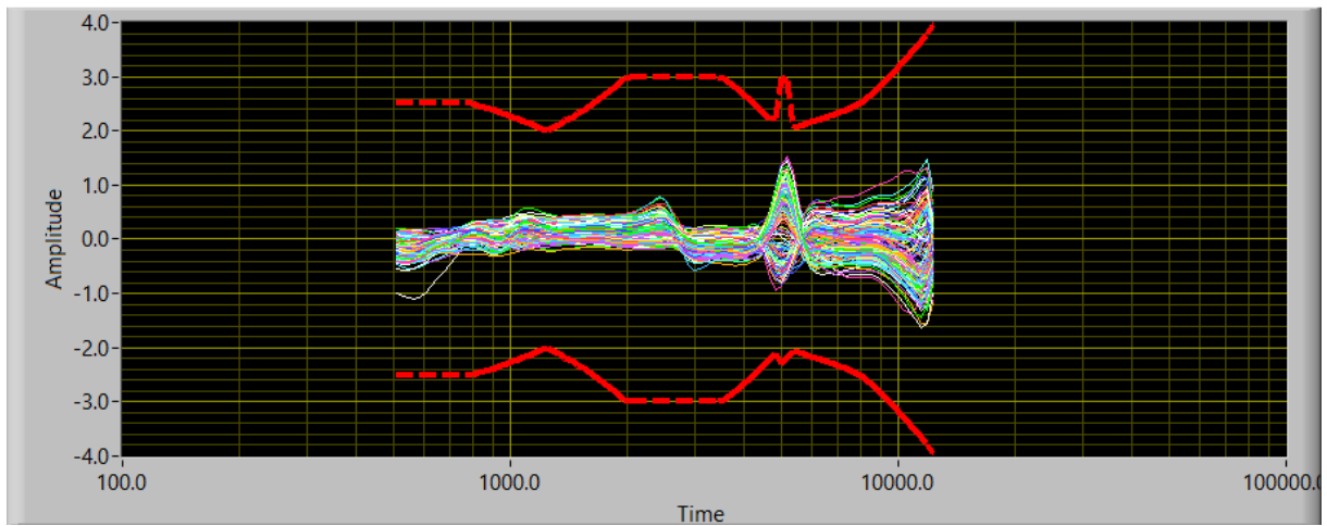
Figure2 All Curve - New Limits
