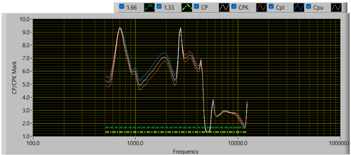
Figure3 CP/CPK - New Limits
