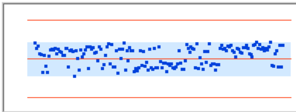
Figure134 Distribution 4835.6670Hz
